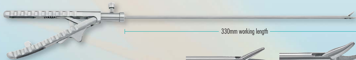
Dick TC Endoscopic Needle Holder, traditional ratchet design, spring loaded handle
